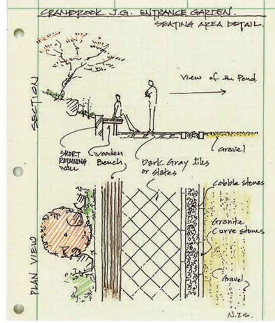
Seating Area detail cross section
